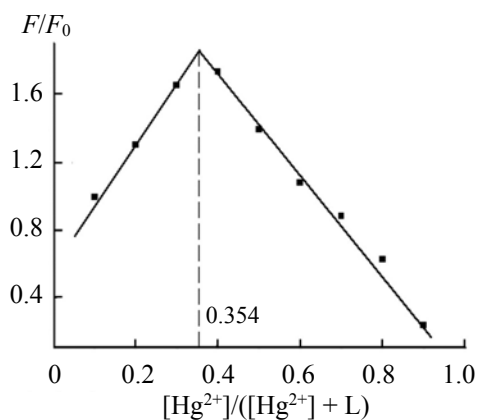
Fig. 4. Job's plot at 526 nm for determining the stoichiometry of HL and \text{Hg}^{2+} in solution (DMF/tris-HCl buffer, 1:1, v/v, pH 7.2).
