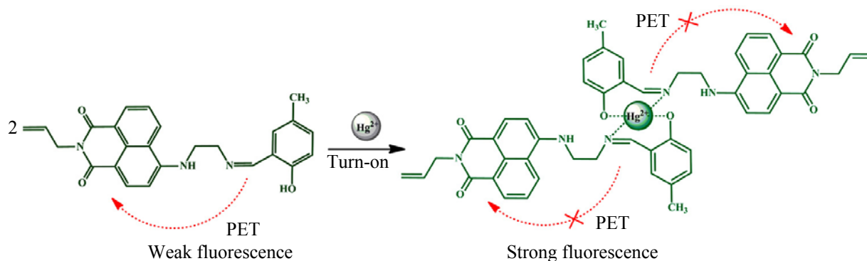
Scheme 2. Proposed binding model of HL with \text{Hg}^{2+} .
