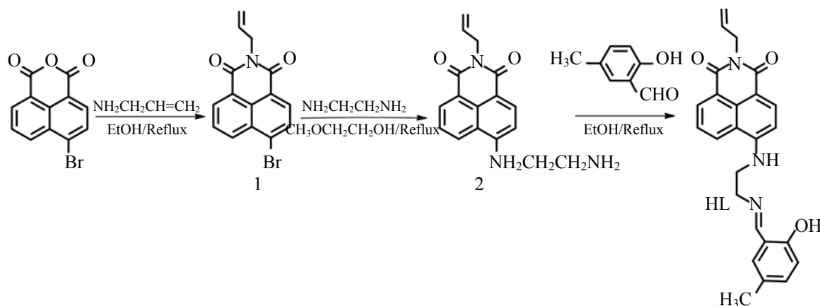
Scheme 1. Chemical structure and synthetic routine of HL.
