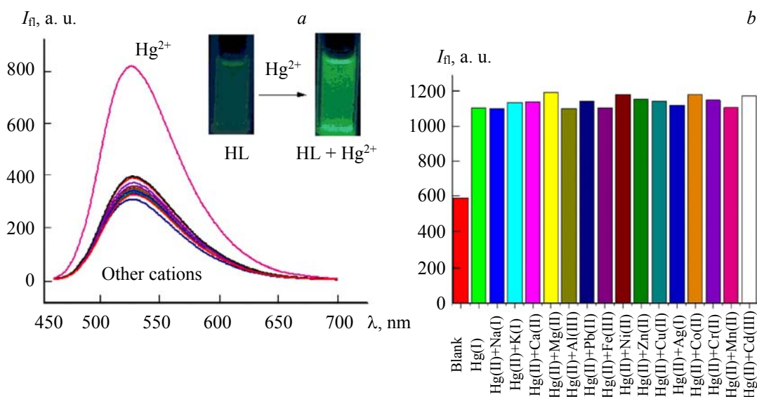
Fig. 2. a) Fluorescence spectra of HL ( 10 \mu\text{M} ) in solution (DMF/tris-HCl buffer, 1:1, v/v, pH 7.2) toward \text{Na}^+ , \text{K}^+ , \text{Ca}^{2+} , \text{Mg}^{2+} , \text{Al}^{3+} , \text{Pb}^{2+} , \text{Fe}^{3+} , \text{Ni}^{2+} , \text{Zn}^{2+} , \text{Cu}^{2+} , \text{Hg}^{2+} , \text{Ag}^+ , \text{Co}^{2+} , \text{Cr}^{3+} , \text{Mn}^{2+} , and \text{Cd}^{2+} with an excitation at 430 nm; b) Competitive experiments in the compound HL+ \text{Hg}^{2+} system with interfering metal ions at 526 nm.
