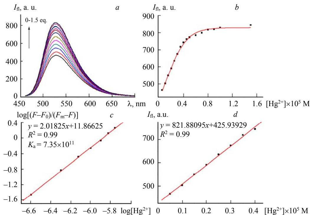
Fig. 3. a) Fluorescence titration spectra of HL with \text{Hg}^{2+} (0–1.5 eq) in solution (DMF/tris-HCl buffer, 1:1, v/v, pH 7.2) at room temperature with an excitation of 430 nm; b) Fitting of the fluorescence titration curve of HL in solution (DMF/tris-HCl buffer, 1:1, v/v, pH 7.2); c) Benesi–Hildebrand linear analysis plots of HL at different \text{Hg}^{2+} concentrations; d) Curve of fluorescence intensity at 526 nm of HL ( 1 \times 10^{-5} \text{ M} ) versus increasing concentrations of \text{Hg}^{2+} ( 0.5\text{--}4.0 \mu\text{M} ).
