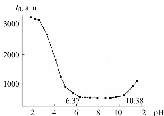
Fig. 1. Fluorescent behavior of HL at different pH values ( \lambda_{\text{exc}} = 430 \text{ nm} , 25^\circ\text{C} ).
