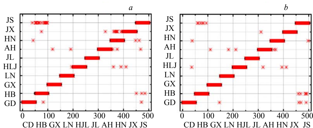
Fig. 3. Classification result of 10 kinds of rice using the support vector machine model by (a) a single spectral line and (b) a multi-spectral line combination. Actual label (●), label predicted by the SVM model (*). The successful classification is achieved when the “*” overlaps with the “●.”
