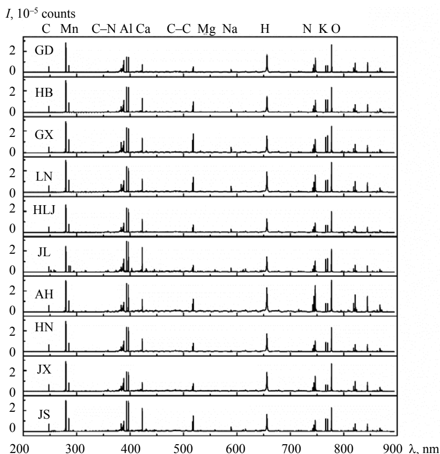
Fig. 2. Laser-induced breakdown spectroscopy spectra of 10 different rice samples.
