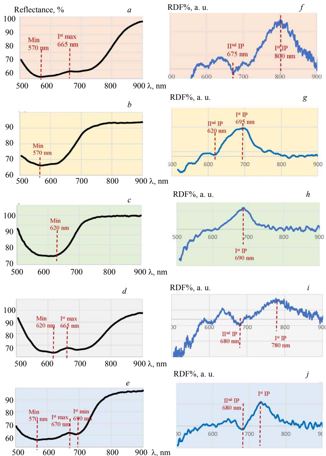
Fig. 4. (a–e) Determination of extrema (also local ones) in the reflectance R\% spectra of Inks 1–5. (f–j) Determination of the well-defined inflection points (extrema in the numerically calculated first derivative of the previous R\% spectra).
