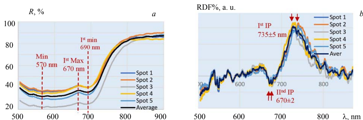
Fig. 2. (a) Repeatability of the reflectance features presented with five reflectance spectra taken from five different sampling spots of the same InkX and their average, and determination of overall minimum in the reflectance spectrum at 570 nm and local maximum in the reflectance well (bottom of the reflectance spectrum) at 670 nm. (b) Determination of inflexion points (extrema in the numerical first derivative of the individual R\% spectra) and their average FD R\% .
