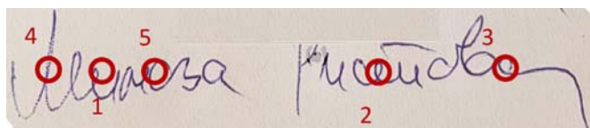
Fig. 1. A nondestructive method for signature ink analysis: Reflectance ( R\% ) spectra were acquired from five sampling points/spots of the signature (ink deposited on white paper). A magnifying glass was used to focus on the chosen sampling spot.
