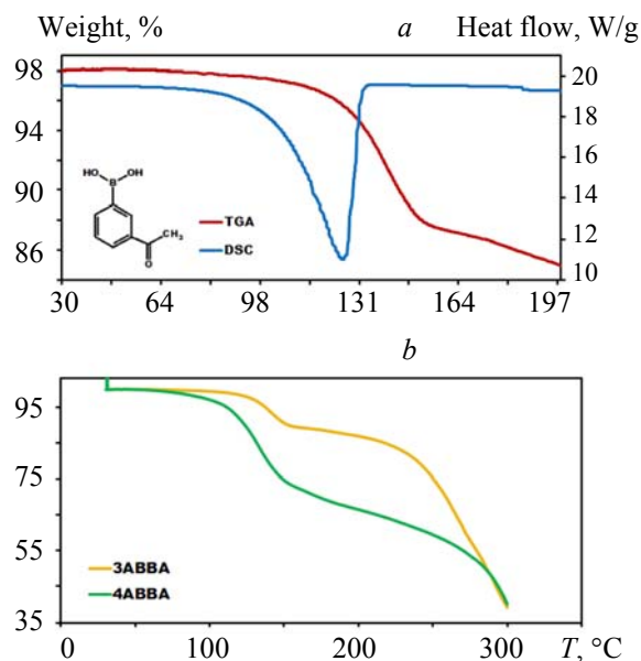
Fig. 5. DSC curve (blue) and TGA curve (red) of 7 (a). Overlay of thermograms of samples 7 and 8 (b). Experimental conditions as in DSC measurements and TGA measurements subsections.
