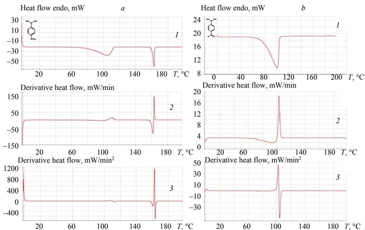
Fig. 4. The hydrolytic stabilities (DSC curves) of 3 (a) and 6 (b) under N_2 atmosphere. Heat flow endo up (mW) versus temperature graph (1), first derivative of heat flow (mW/min) versus temperature curve (2), second derivative of heat flow (mW/min 2 ) versus temperature plot (3). 4.0 mg of sample placed in hermetically sealed aluminum pans. Heating-cooling-heating cycle was in temperature range 0–225°C (50°C/min ramping rate).
