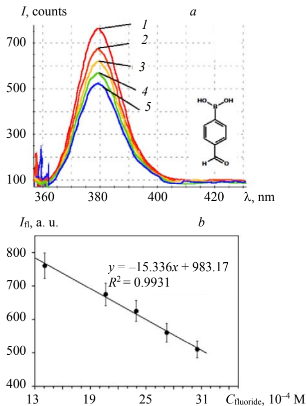
Fig. 7. Fluorescence quenching of 6 with 1400 (1), 2000 (2), 2300 (3), 2700 (4), 3000 \mu M (5) fluoride. Experimental conditions as in the spectrofluorimetry experiments subsection.
