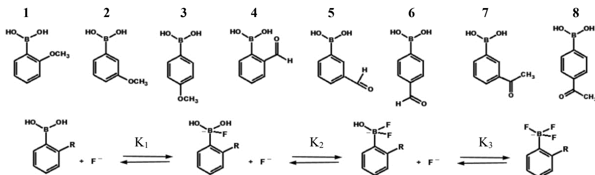
Fig. 1. Numbering and structures of compounds; ortho - (1), meta - (2) and para - (3) methoxyphenyl-BAs, ortho - (4), meta - (5), and para - (6) formylphenyl-BAs, meta - (7) and para - (8) acetylphenyl-BAs. Proposed reaction scheme for fluoride complexation of BAs, for quantification.
