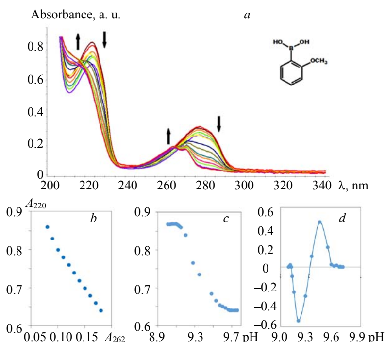
Fig. 2. Titration of 10^{-3} M 1 with 10^{-3} M NaOH (a). Graphs of dependence of absorbance at 220 nm on absorbance at 262 nm (b), on medium pH (c) and dependence of the ratio of second derivation of absorbance to second derivation of titrant volume on pH (d). Experimental conditions as in spectrophotometric pK_a .
