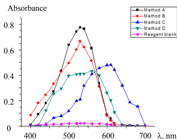
Fig. 1. Absorption spectra of DEX.HCl with amaranth dye (8 µg/mL) (method A), safranin dye (9.0 µg/mL) (method B), aniline blue (6 µg/mL) (method C), rhodamine B (2.4 µg/mL) (method D) against reagent blank.
