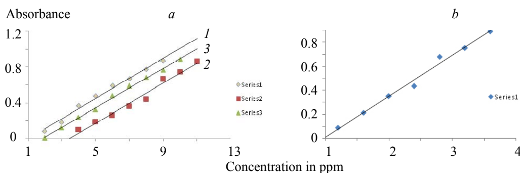
Fig. 2. Beer's law curves of DEX.HCl: a – with amaranth (1), safranin (2), and aniline blue (3) for methods A, B, and C; b – with rhodamine B (method D).
