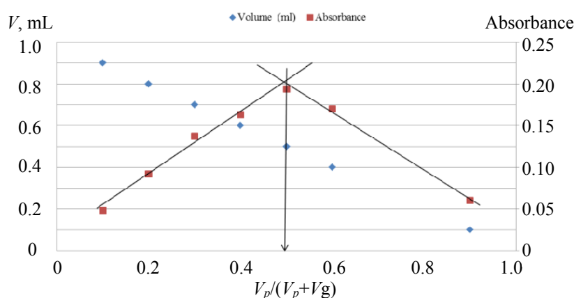
Fig. 4. The continuous variation plot of the complex.
