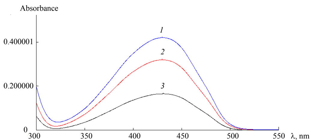
Fig. 2. UV/Vis spectra of the metoclopramide hydrochloride solution 5.5 (1), 4.0 (2), and 2.0 \mu\text{g/mL} (3) after diazotization and coupling with dimethylphenol.
