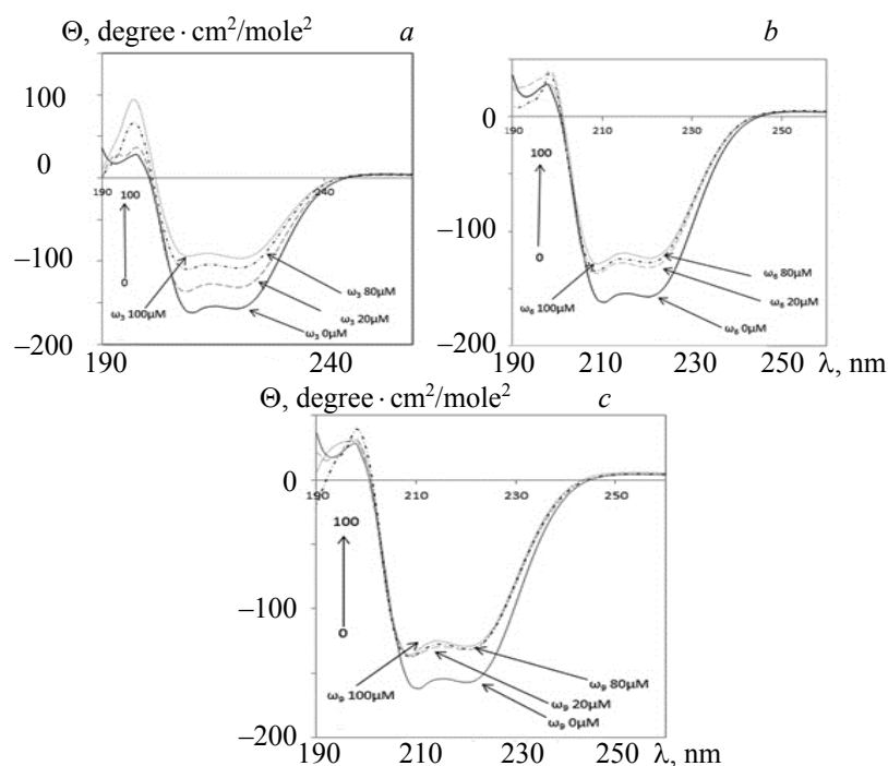
Fig. 5. Far-UV-CD spectra of the HSA/omega3-6-9 fatty acid interaction: HSA = 40 \mu\text{M} and omega-3-6-9 = 0, 20, 80, and 100 \mu\text{M} .
