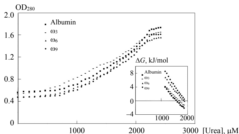
Fig. 1. UV/vis absorbance spectra of chemical denaturation after titration by urea in the concentration of HSA 40 \mu M and its interaction with omega-3, omega-6, and omega-9. Inset: secondary plot of the two state chemical denaturation.
