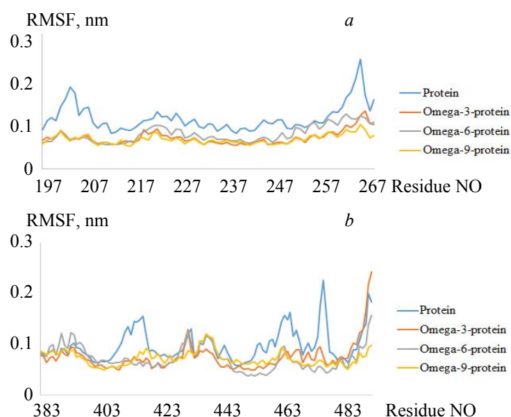
Fig. 8. The RMSF values of free HSA and HSA in complex with omega-3, omega-6, and omega-9 in site I/II (a/b).
