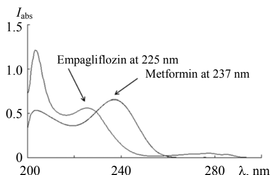
Fig. 1. Overlay of the absorption spectra of EG (8 \mu\text{g}/\text{mL} ) and MT (8 \mu\text{g}/\text{mL} ), using methanol as a blank.
