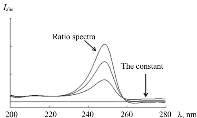
Fig. 2. The obtained ratio spectra of 2–12 \mu\text{g}/\text{mL} MT divided by 12 \mu\text{g}/\text{mL} EG in methanol.
