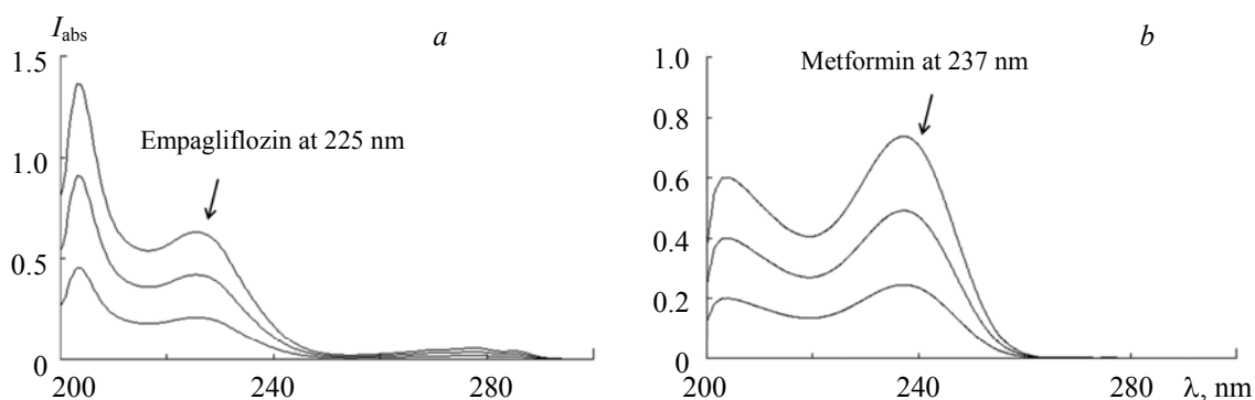
Fig. 3. The obtained EG (a) and MT (b) zero-order spectra (3, 6, and 9 \mu\text{g/mL} ) resolved from the laboratory prepared mixtures using CM (a) and SS method (b).
